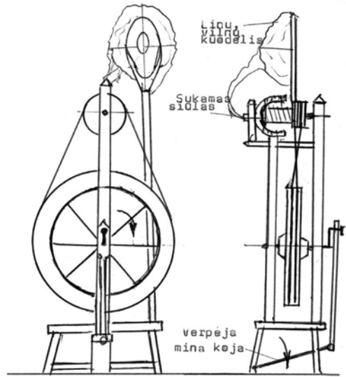
Verpimo ratelis
